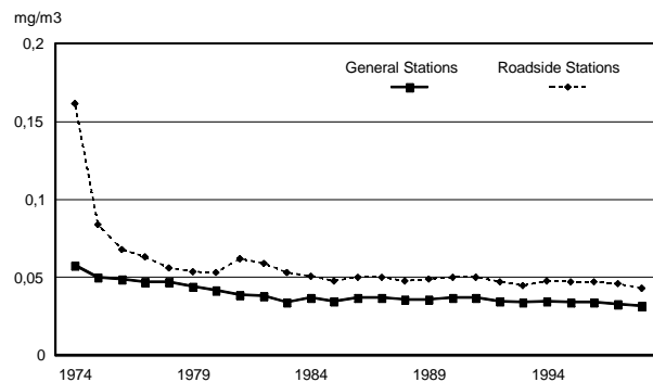
Suspended Particulate Matter Air Quality Trends In Japan
