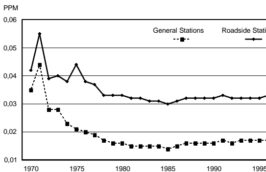
Nitrogen Dioxide Air Quality Trends In Japan
